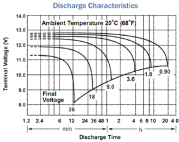
Power-Sonic's expected performance for a typical 18Ah AGM battery. Some working conditions might necessitate a 35 Ah battery instead. This chart is based on the "20 hour rate" of discharge. Note the logarithmic axis. Power-sonic Model PS-12180
