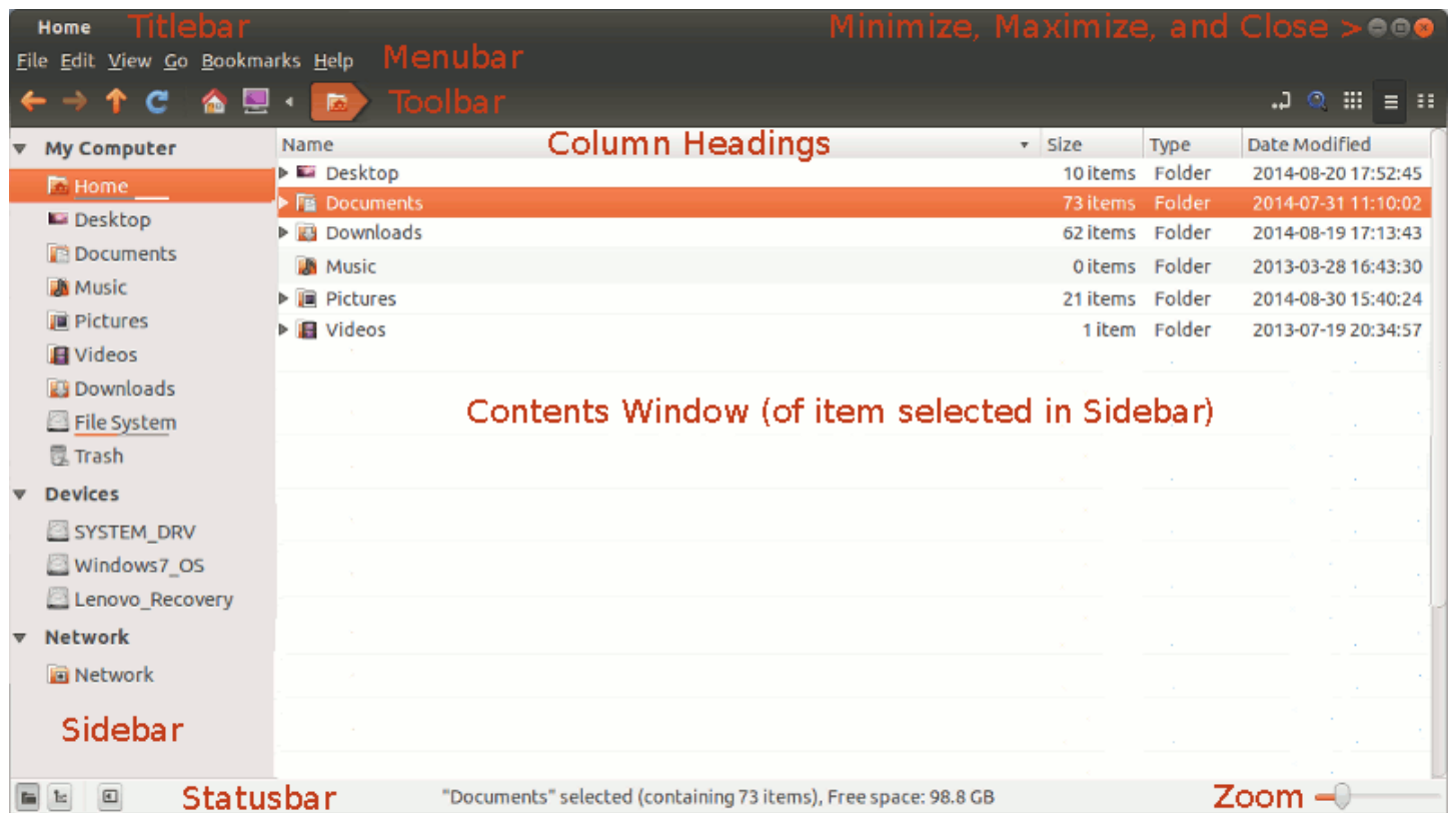
The File Manager (with labels)
